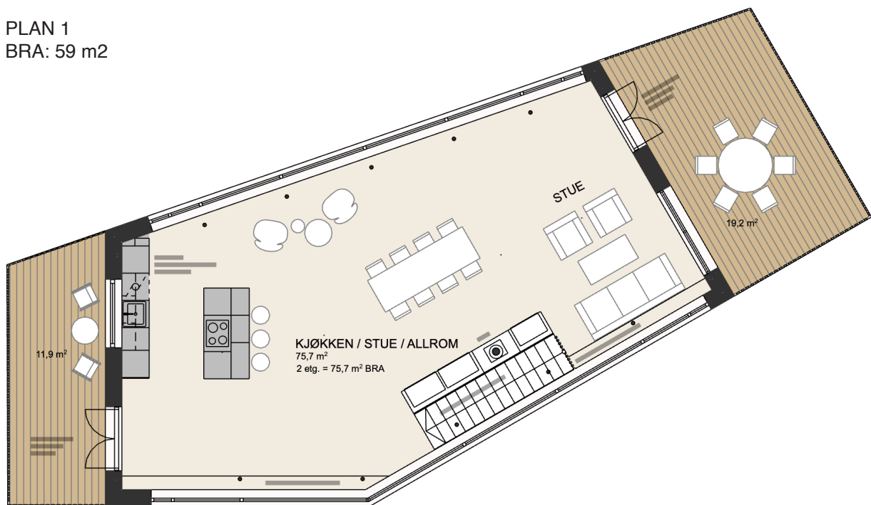
PLAN 2 BRA: 75 m2
